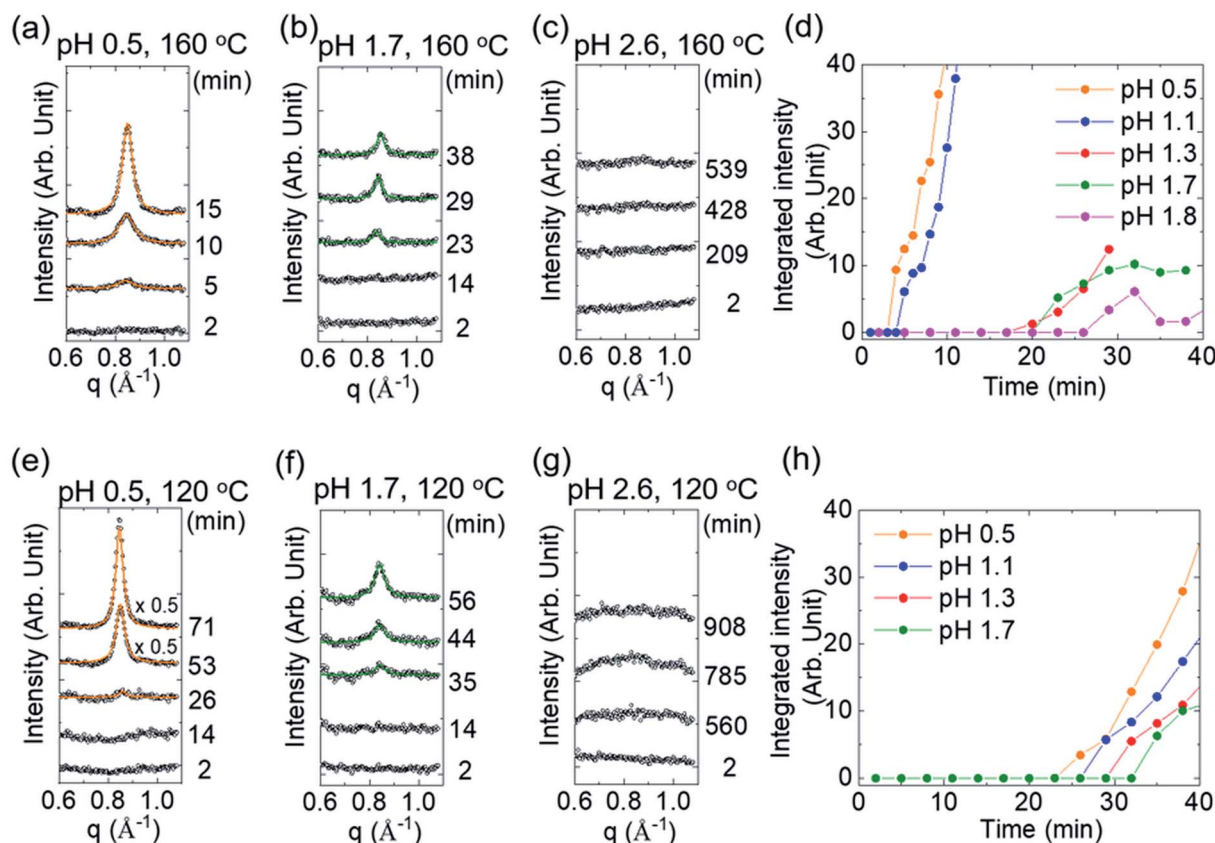
Fig. 2 Evolution of the \delta' - \text{MnO}_2 (200) peak and onset of crystallization. The \delta' - \text{MnO}_2 (200) peak evolution at representative pH and time points at 160 °C (a–c) and 120 °C (e–g), showing the onset point and intensity growth after. The experimental data and the fits are shown by the open circles and solid lines, respectively. The onset of \delta' - \text{MnO}_2 is defined as the time point that the (200) peak shape can be meaningfully fitted by a Lorentzian function. The integrated intensity of the (200) scattering peak in the first 40 min of the hydrothermal reaction at 160 °C (d) and 120 °C (h). For the data after 40 min and not presented here in the manuscript, please see Fig. S2 in ESI 3†
