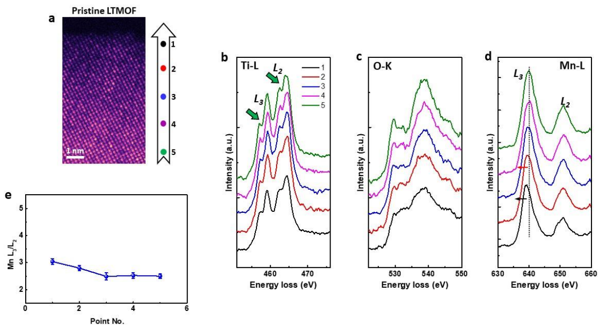
Figure S12. (a) STEM HAADF image of pristine LTMOF, which is same as Fig. 2(e). (b–d) EELS spectra collected at 5 different locations below the surface of pristine LTMOF, marked by the points in (a). (e) Mn L 3 /L 2 ratios measured at the 5 different locations.
