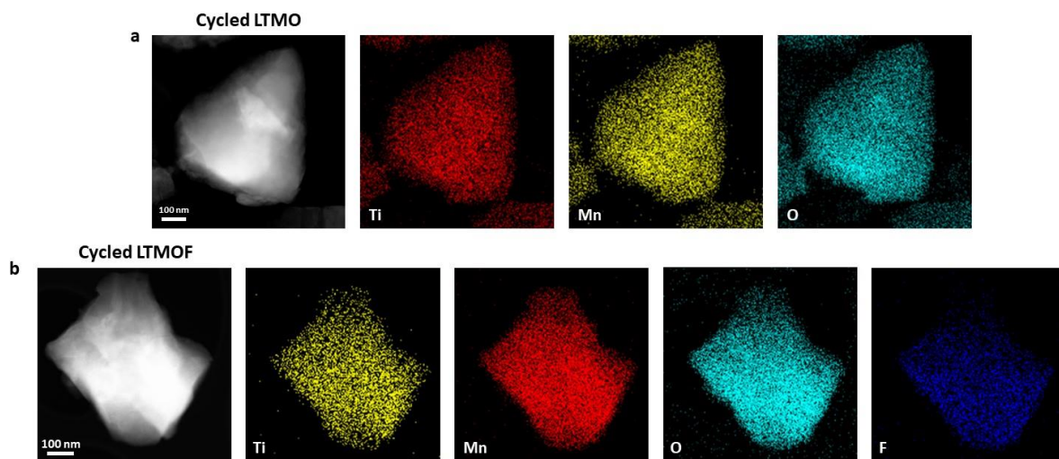
Figure S4. STEM image and corresponding EDS elemental maps of LTMO (a) and LTMOF (b) particles after 50 cycles.
