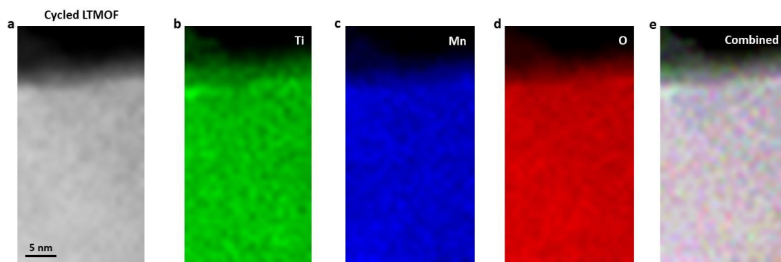
Figure S10. STEM image (a) and corresponding EELS elemental maps (b–e) of a nanoscale surface region in LTMOF after 50 cycles.
