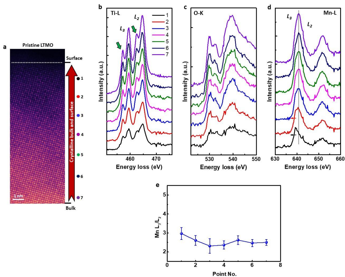
Figure S7. (a) STEM HAADF image of pristine LTMO, which is same as Fig. 2(a). (b–d) EELS spectra collected at 7 different locations below the surface of pristine LTMO, marked by the points in (a). (e) Mn L_3/L_2 ratios measured at the 7 different locations.
