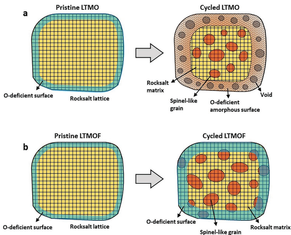
Figure 5. Schematic illustration of structural and chemical evolution in LTMO and LTMOF induced by cycling. a) In LTMO, electrochemical cycling results in surface degradation, such as amorphization and void formation, and rocksalt-to-spinel-like structural transformation within nanosized grains dispersed in the DRX matrix. b) In LTMOF, electrochemical cycling results in rocksalt-to-spinel-like structural transformation within nanosized grains dispersed in the DRX matrix, whereas the crystalline surface remains well preserved.
