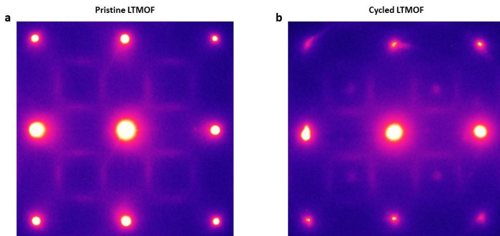
Figure S15. Electron diffraction patterns for pristine LTMOF (a) and discharged LTMOF after 50 cycles (b).
