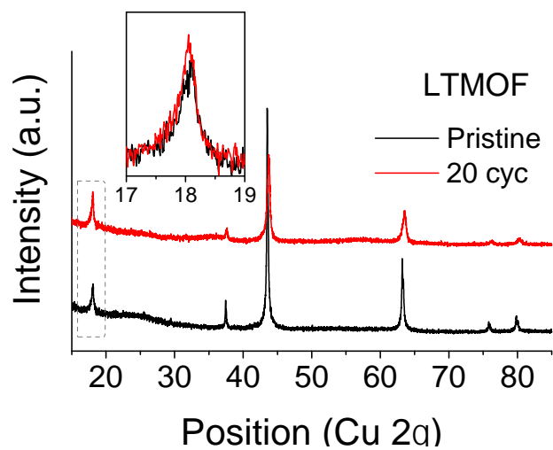
Figure S16. XRD patterns of pristine and cycled (after 20 cycles) LTMOF electrode films (with active materials, carbon black and PTFE binder).
