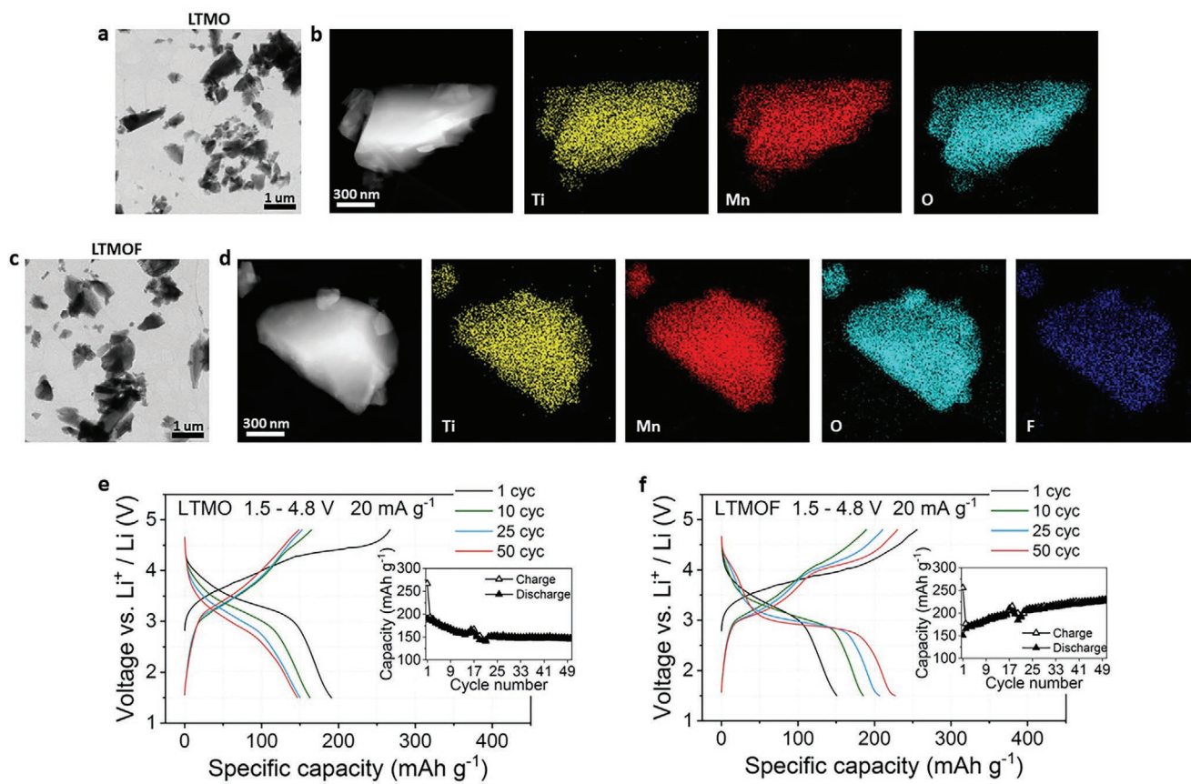
Figure 1. Morphology, composition, and electrochemical properties of LTMO and LTMOF particles. a) TEM image of pristine LTMO particles. b) STEM image and corresponding EDS elemental maps of a pristine LTMO particle. c) TEM image of pristine LTMOF particles. d) STEM image and corresponding EDS elemental maps of a pristine LTMOF particle. e,f) Charge and discharge voltage profiles for the 1st, 10th, 25th, and 50th cycles and specific capacity as a function of cycle number (inset) for LTMO (e) and LTMOF (f) cathodes in half-cells cycled between 1.5 and 4.8 V at a current density of 20 mA g -1 . The capacity fluctuation near the 18th cycle in both tests was caused by unintended temperature fluctuation.
