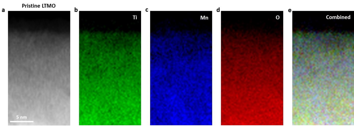
Figure S5. STEM image (a) and corresponding EELS elemental maps (b–e) of a nanoscale surface region in pristine LTMO.
