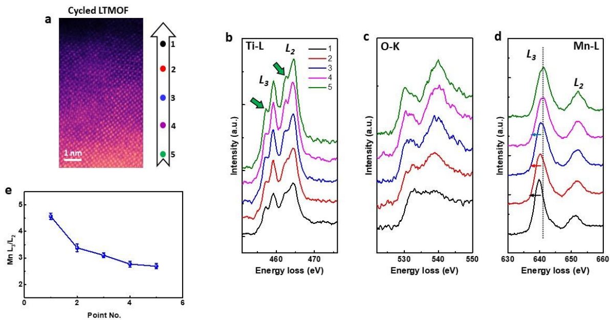
Figure S13. (a) STEM HAADF image of LTMOF after 50 cycles, which is same as Fig. 2(f). (b–d) EELS spectra collected at 5 different locations below the surface of cycled LTMOF, marked by the points in (a). (e) Mn L_3/L_2 ratios measured at the 5 different locations.
