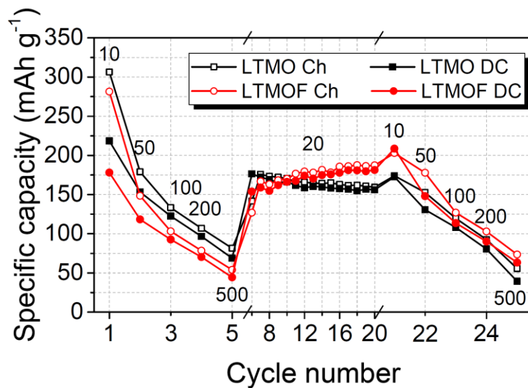
Figure S17. Rate capability measurements of the LTMO and LTMOF cathodes. For both cells, the 1 st to 5 th cycles were measured at 10, 50, 100, 200, 500 mA g -1 , respectively; the 6 th to 20 th cycle were cycled at 20 mA g -1 ; the 21 st to 25 th cycles were measured at 10, 50, 100, 200, 500 mA g -1 , respectively again.
