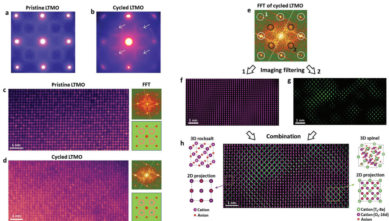
Figure 3. Structural transformation in LTMO cathode induced by cycling. a,b) Electron diffraction patterns for pristine LTMO (a) and discharged LTMO after 50 cycles (b). The white arrows in (b) mark the 4 additional spots corresponding to the spinel-like lattice. c) Atomic-resolution STEM HAADF image of a nanoscale bulk region in pristine LTMO (left), corresponding FFT (top right), and schematic for the FFT (bottom right). d) Atomic-resolution STEM HAADF image of a nanoscale bulk region in discharged LTMO after 50 cycles (left), corresponding FFT (top right), and schematic for the FFT (bottom right). e–h) Procedures and results of STEM HAADF image filtering. In the FFT (e), white-colored filtering masks that only allow structural information from the rocksalt cubic lattice were applied, and an inverse Fourier transform was performed, resulting in a filtered image (f) that only contains rocksalt structures. Black-colored filtering masks that only allow structural information from the spinel-like lattice were applied, and an inverse Fourier transform was performed, resulting in a filtered image (g) that only contains spinel-like structures. A combination of (f) and (g) results in a single filtered image (h) showing the spatial distribution of rocksalt (purple) and spinel-like (green) structures. 3D and 2D atomic models of rocksalt and spinel structures are shown on the left and right sides of the filtered image, respectively.
