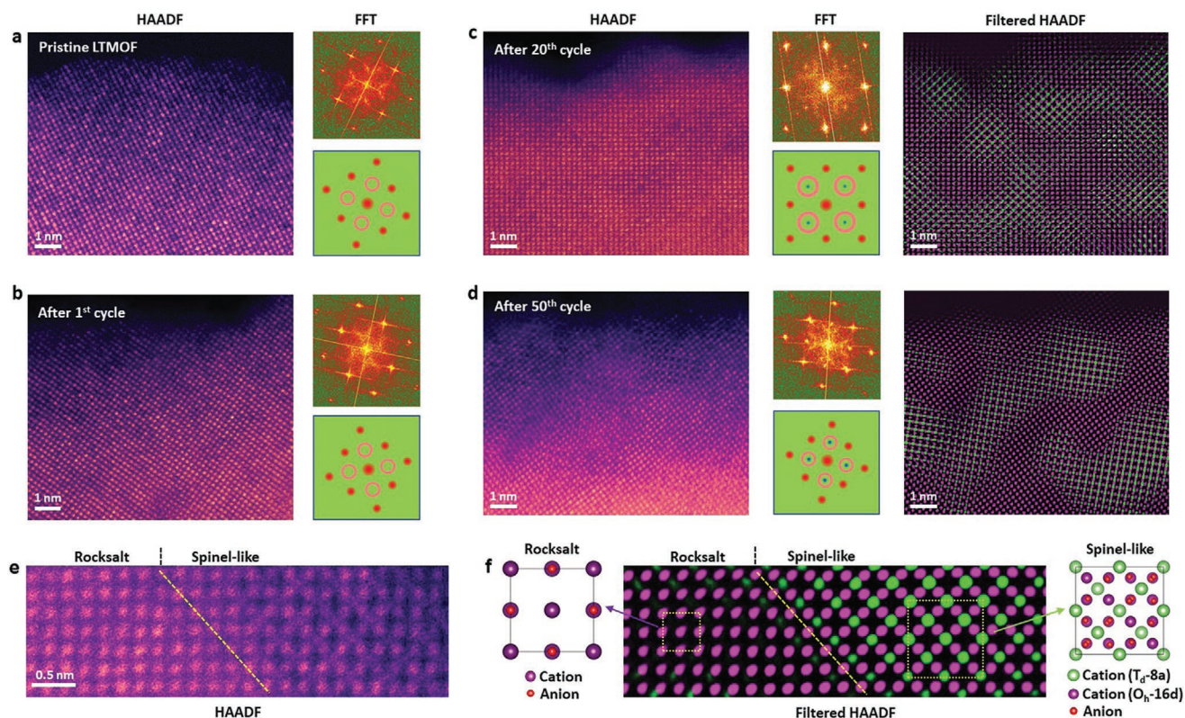
Figure 4. Structural transformation in LTMOF cathode induced by cycling. a) Atomic-resolution STEM HAADF image of a nanoscale region in pristine LTMOF (left), corresponding FFT (top right), and schematic for the FFT (bottom right). b) Atomic-resolution STEM HAADF image of a nanoscale region in discharged LTMOF after the 1st cycle (left), corresponding FFT (top right), and schematic for the FFT (bottom right). c) Atomic-resolution STEM HAADF image of a nanoscale region in discharged LTMOF after 20 cycles (left), corresponding FFT (top middle), schematic for the FFT (bottom middle), and corresponding filtered STEM HAADF image (right) showing the spatial distribution of rocksalt (purple) and spinel-like (green) structures. d) Atomic-resolution STEM HAADF image of a nanoscale region in discharged LTMOF after 50 cycles (left), corresponding FFT (top middle), schematic for the FFT (bottom middle), and corresponding filtered STEM HAADF image (right) showing the spatial distribution of rocksalt (purple) and spinel-like (green) structures. e) Magnified STEM HAADF image of a boundary across rocksalt and spinel-like structures in cycled LTMOF. f) Corresponding filtered image of the magnified STEM HAADF image in (e), showing the spatial distribution of rocksalt (purple) and spinel-like (green) structures. 2D atomic models of rocksalt and spinel structures are shown on the left and right sides of the filtered image, respectively.
