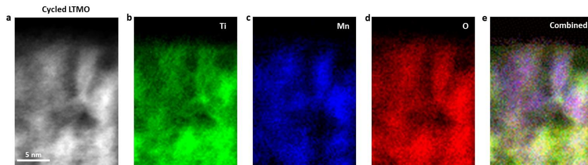
Figure S6. STEM image (a) and corresponding EELS elemental maps (b–e) of a nanoscale surface region in LTMO after 50 cycles.
