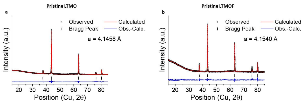
Figure S1. XRD patterns of pristine LTMO (a) and LTMOF (b) cathode particles.
