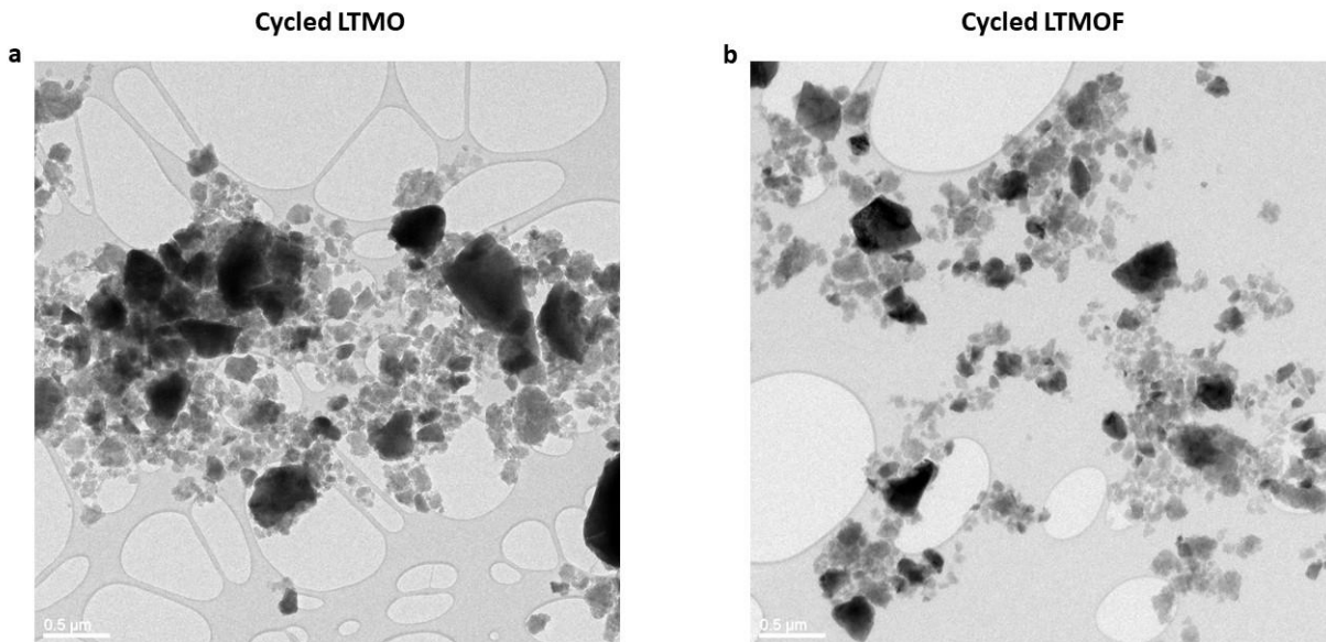
Figure S3. TEM images of LTMO (a) and LTMOF (b) particles after 50 cycles.
