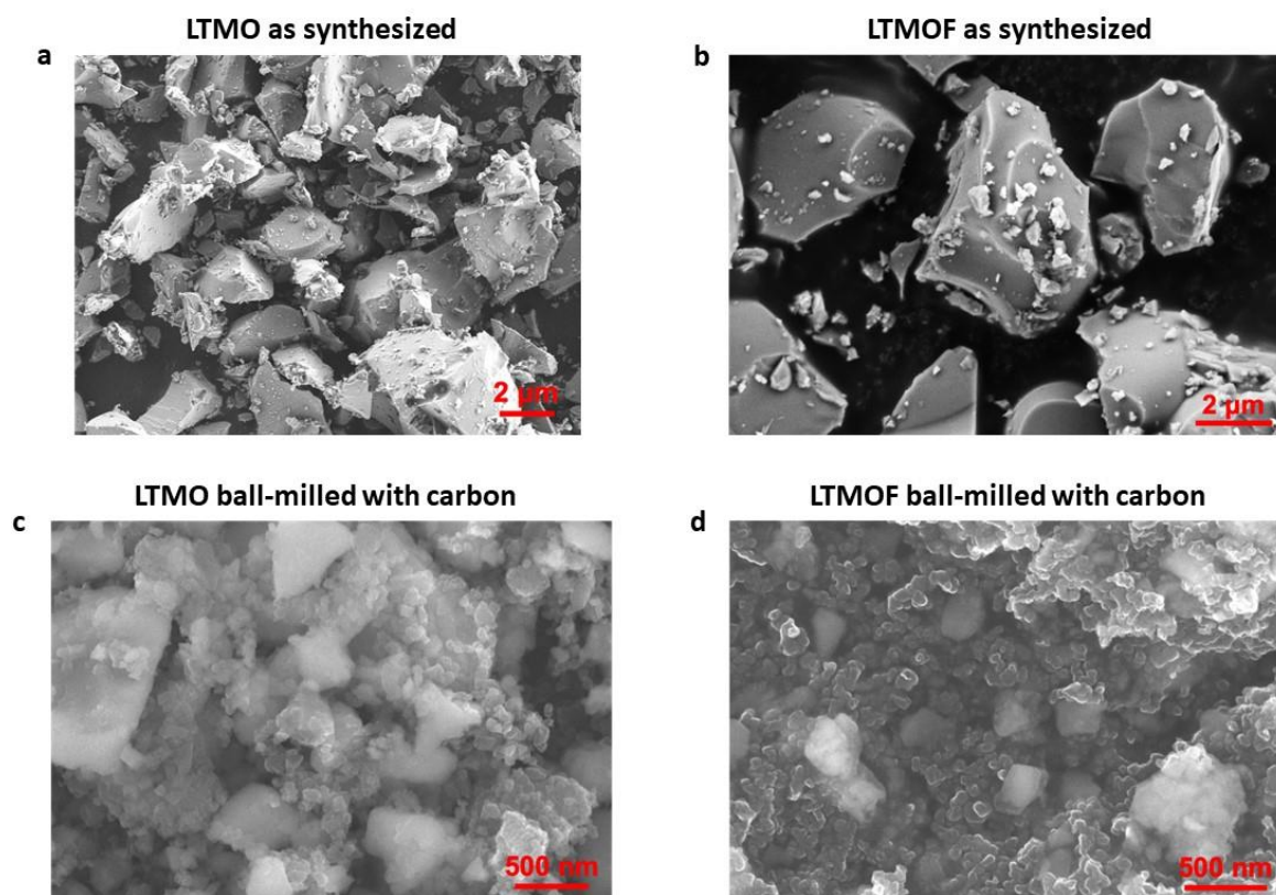
Figure S2. SEM images of as-synthesized LTMO (a) and LTMOF (b) particles and ball-milled LTMO (c) and LTMOF (d) particles.
