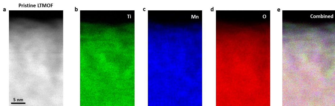
Figure S9. STEM image (a) and corresponding EELS elemental maps (b–e) of a nanoscale surface region in pristine LTMOF.
