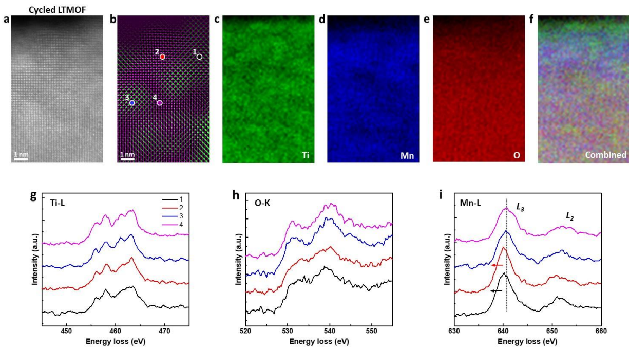
Figure S11. STEM HAADF image (a), corresponding filtered image (b), and corresponding EELS elemental maps (c–f) of a nanoscale surface region in discharged LTMOF after 20 cycles. (g–i) EELS spectra collected at 4 different locations in cycled LTMOF, marked by the points in (b). Note that points 1 and 3 are located within spinel-like structures, and points 2 and 4 are located within rocksalt structures.
