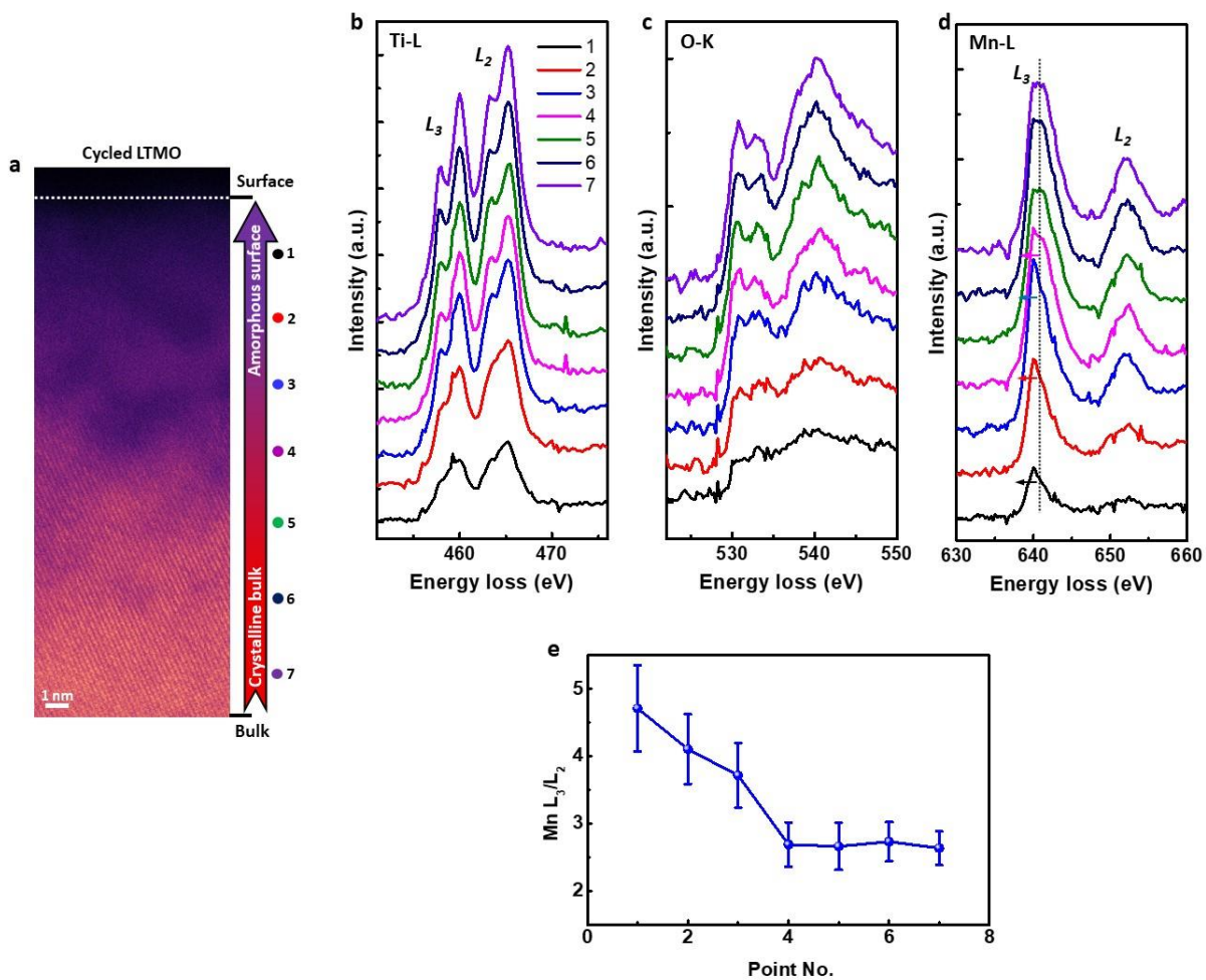
Figure S8. (a) STEM HAADF image of LTMO after 50 cycles, which is same as Fig. 2(b). (b–d) EELS spectra collected at 7 different locations below the surface of cycled LTMO, marked by the points in (a). (e) Mn L_3/L_2 ratios measured at the 7 different locations.
