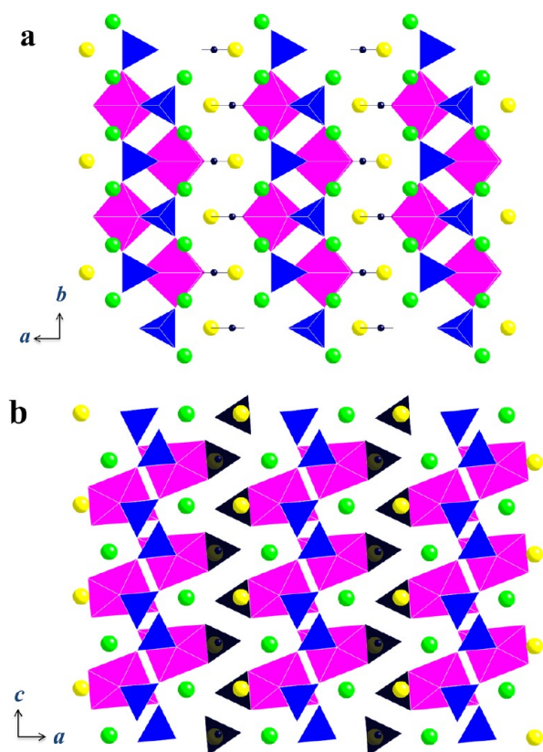
Figure 2. Structure of \text{Na}_3\text{MPO}_4\text{CO}_3 ( \text{M} = \text{Mn}, \text{Fe}, \text{etc.} ) viewed from [001] (a) and [010] (b). Transition metal octahedra, purple; \text{PO}_4 tetrahedra, blue; \text{CO}_3 triangle planar, black; Na, green (Na1) and yellow balls (Na2).
